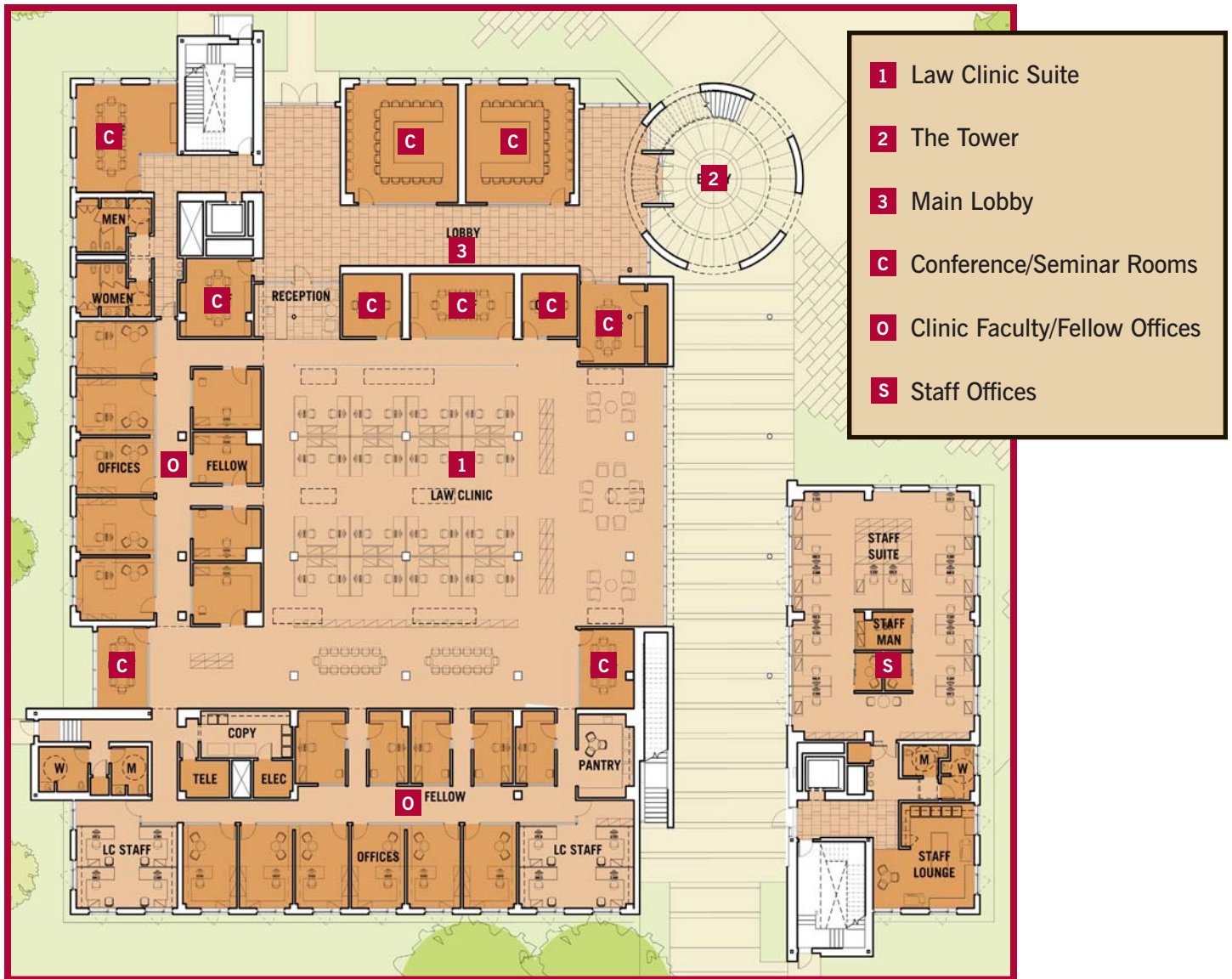
Stanford Law School's New Academic Building Ground Floor
